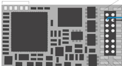
MX645P16 top side (with PluX16)
