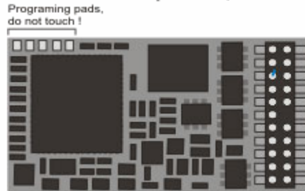
MX645P22 Top View (with PluX22)
