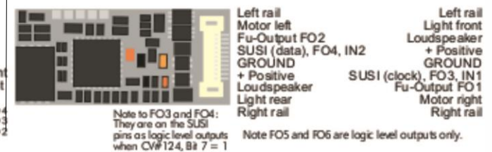
Connector Side (Next 18)
