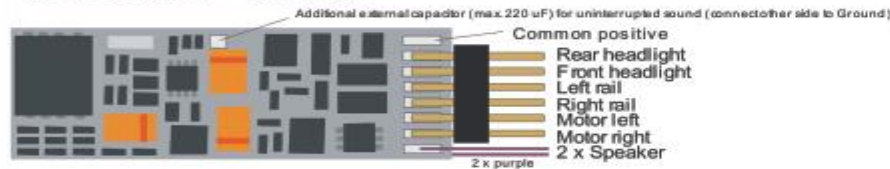
MX 646N, ..W Top Side
